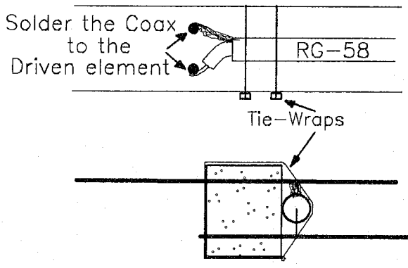
Driven Element Detail
